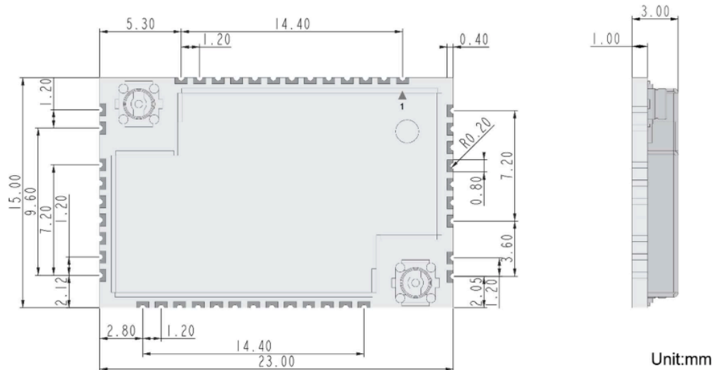
Figure 4: Board dimension
